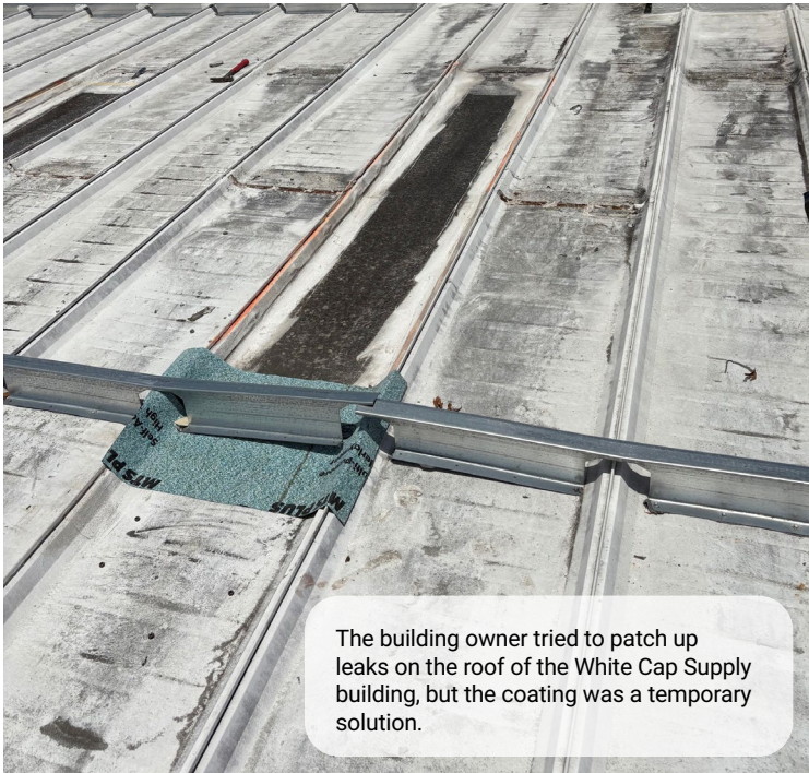
Roof Hugger sub-purlins enabled AWR All Weather Roofing to avoid unnecessary tear-off, cut time and give the owner a more durable energy-efficient system custom-fitted to the existing profile.
