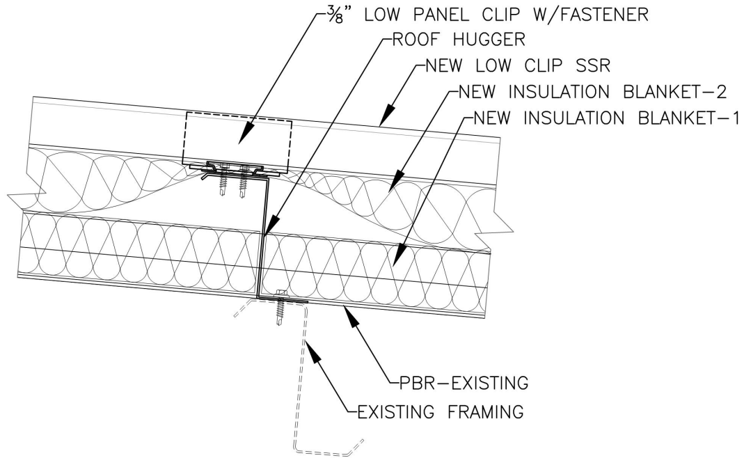
3/8" LOW CLIP W/ NO THERMAL SPACER SSR OVER PBR DOUBLE BLANKET
