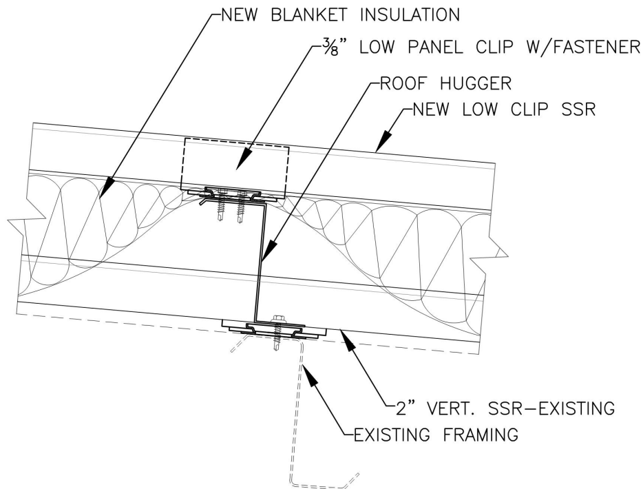
3/8" LOW CLIP SSR OVER SSR SINGLE BLANKET
